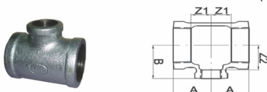
Fig No. 130R - REDUCING TEES BANDED (BRT)
