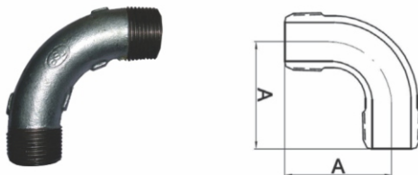
Fig No. 3 - BENDS LONG MALE 90° (MM 90L)
