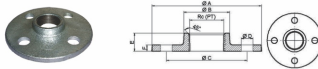
Fig No. 322 - ROUND FLANGES WITH BOLTS HOLE (RF)
