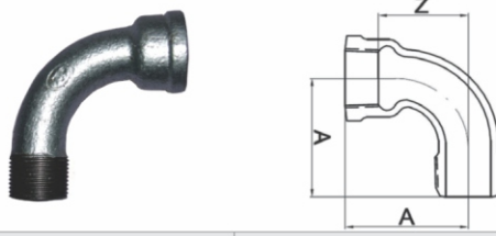
Fig No. 1 - BENDS LONG M&F 90° BANDED (MF 90L)
