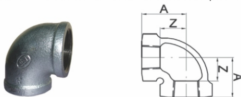
Fig No. 90 - ELBOWS 90° BANDED (BL 90)
