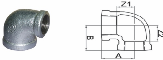
Fig No. 90R - REDUCING ELBOWS 90° BANDED (BRL)
