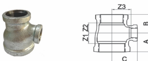
Fig No. 130R - REDUCING TEES BANDED (BRT)
