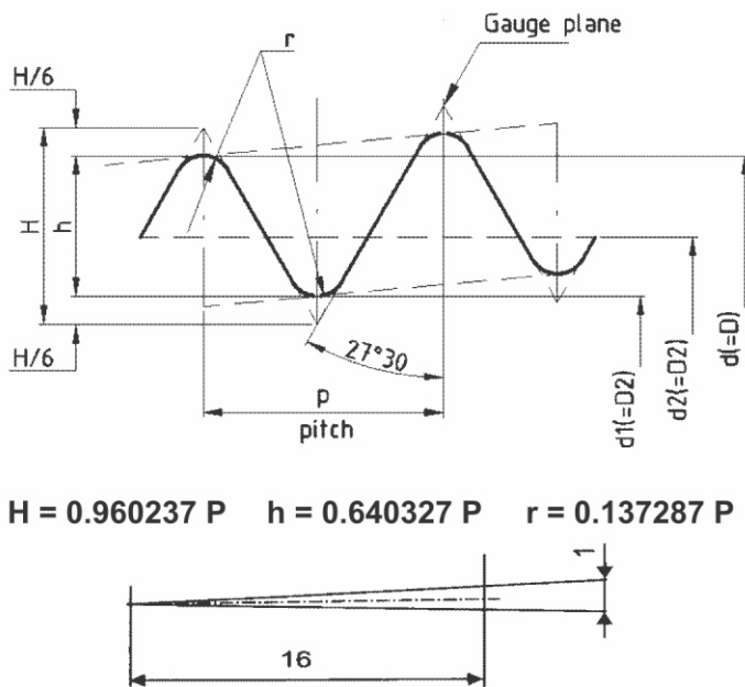
Taper Thread
